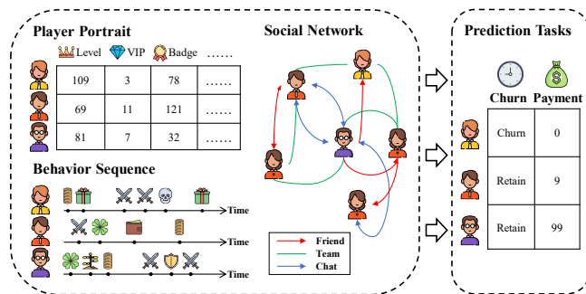
Fig. 1. Illustration of churn and payment prediction based on three heterogeneous data sources in online games. The player portrait describes some players’ attributes. The behavior sequence expresses the event type and time for each in-game action of players, where different icon represents different event. And the social network shows the diverse interactions between players.
